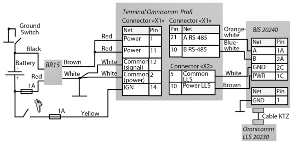
Figure 19. Scheme of connection of the controllable auxiliary equipment
