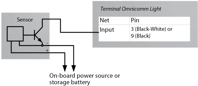
Picture 10. Scheme of connection of the sensor which has a N-P-N output of «open collector» type to the universal input of the Omnicomm Light Terminal
