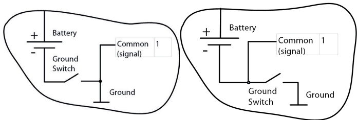
Picture 4. The scheme of connection to the power supply circuit when it is behind the ground switch
